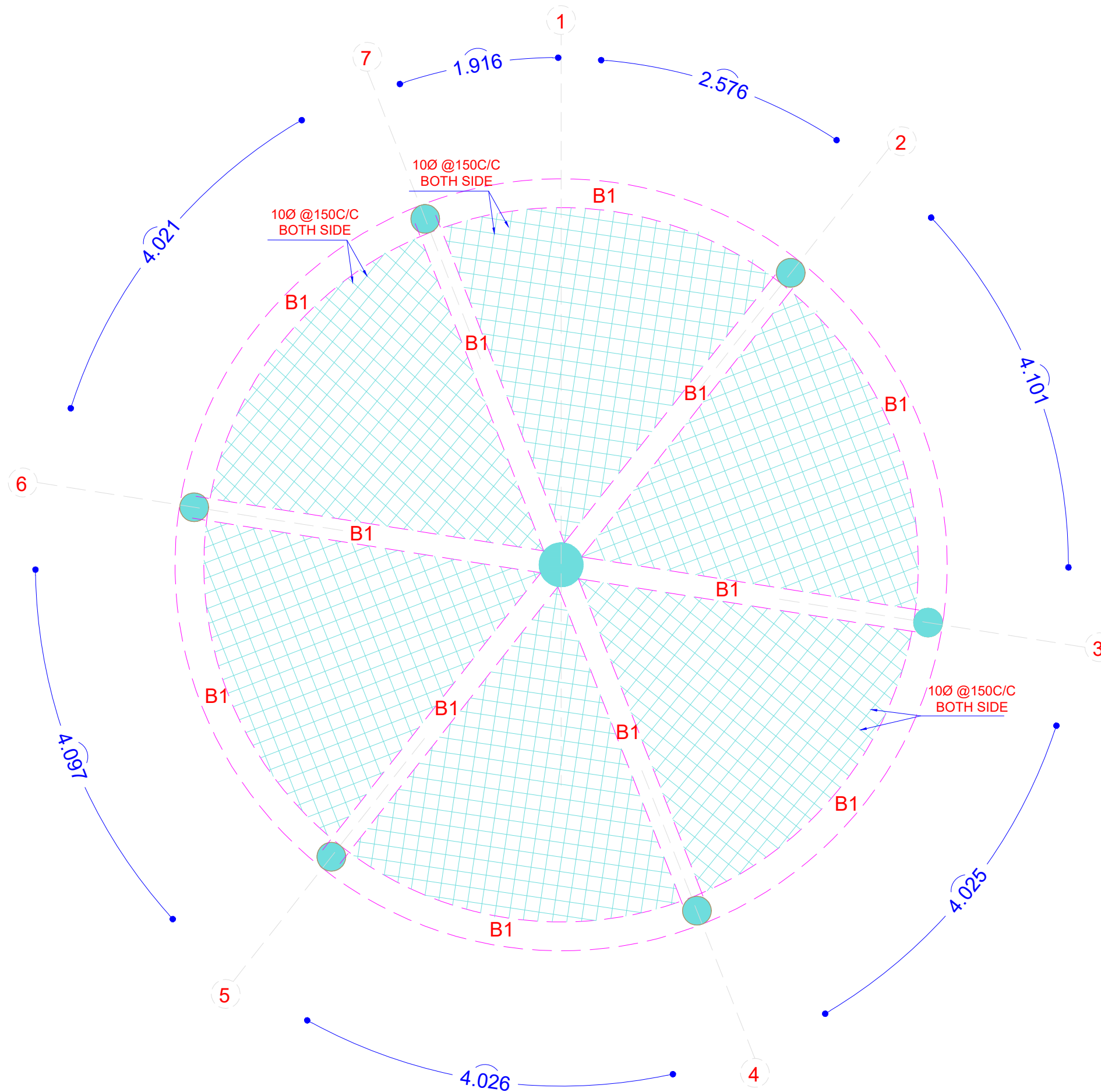
ROOF BEAM PLAN
