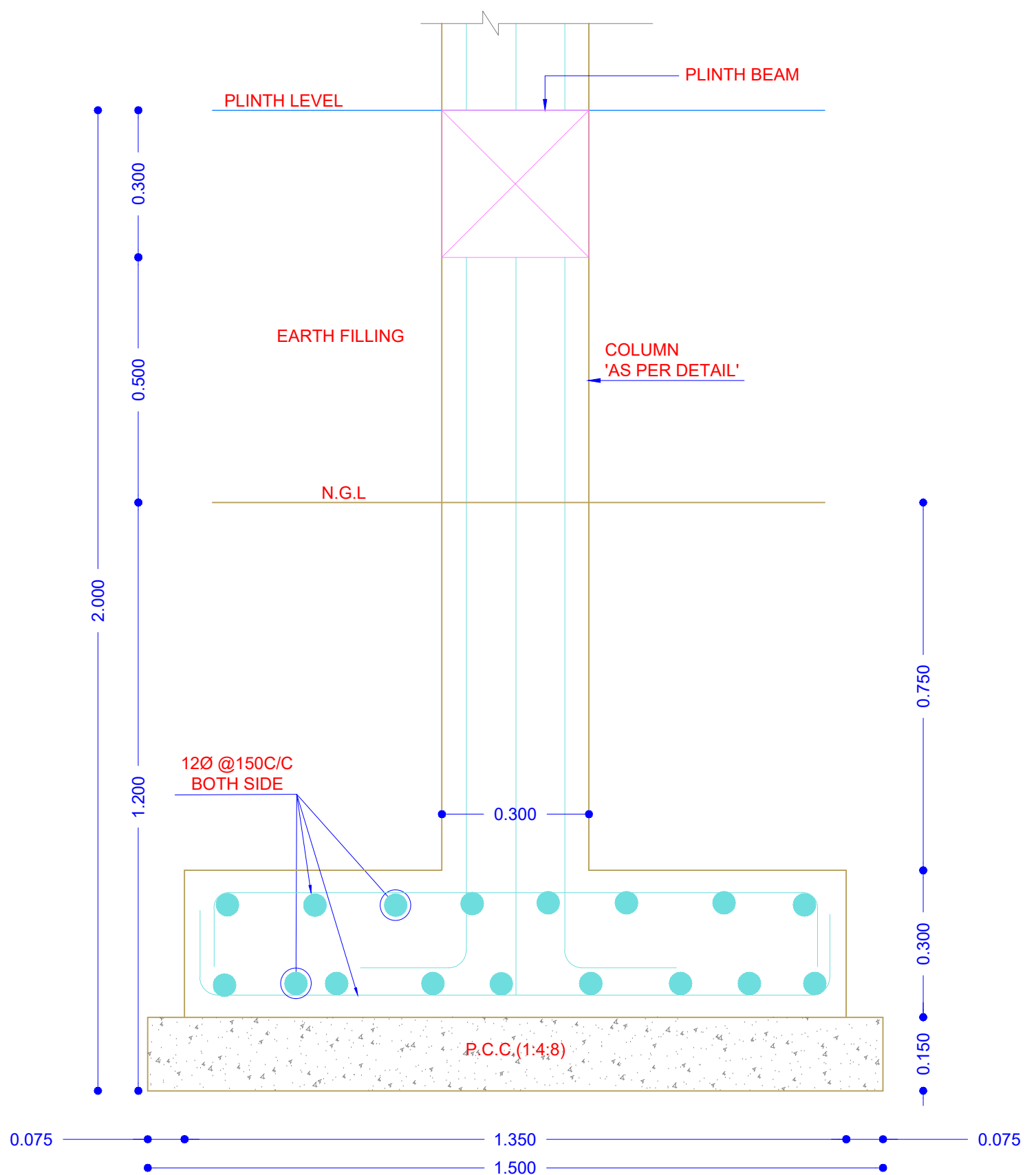
FOOTING DETAIL (F1) 1.500X1.500
